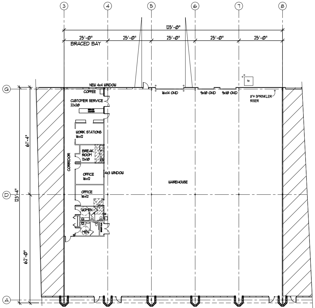
FLOOR PLAN
