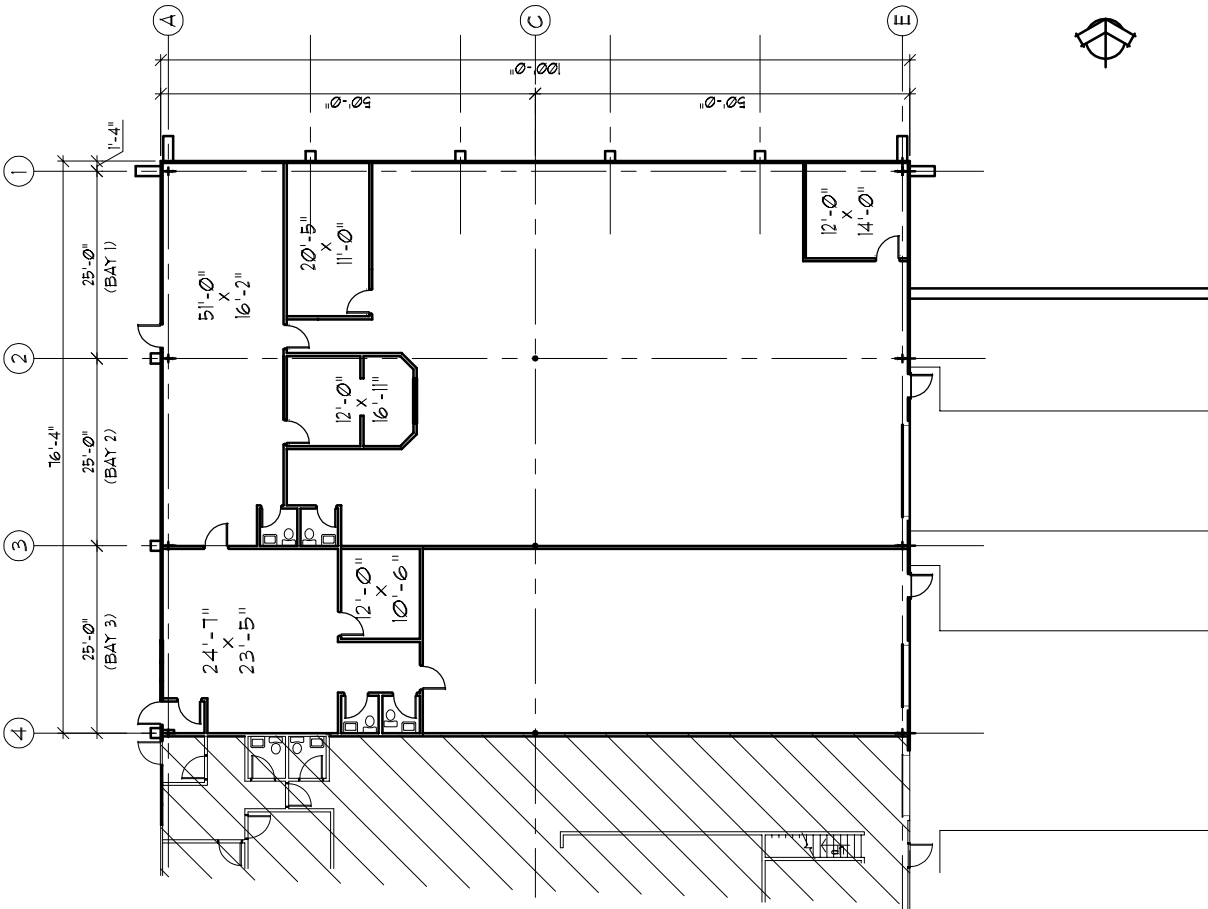
FLOOR PLAN FRAMES 1-4
