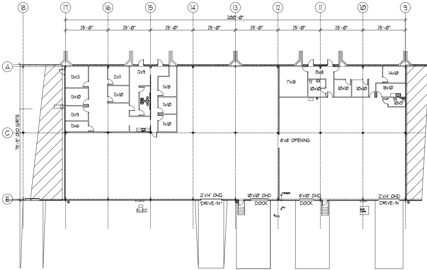
FLOOR PLAN
