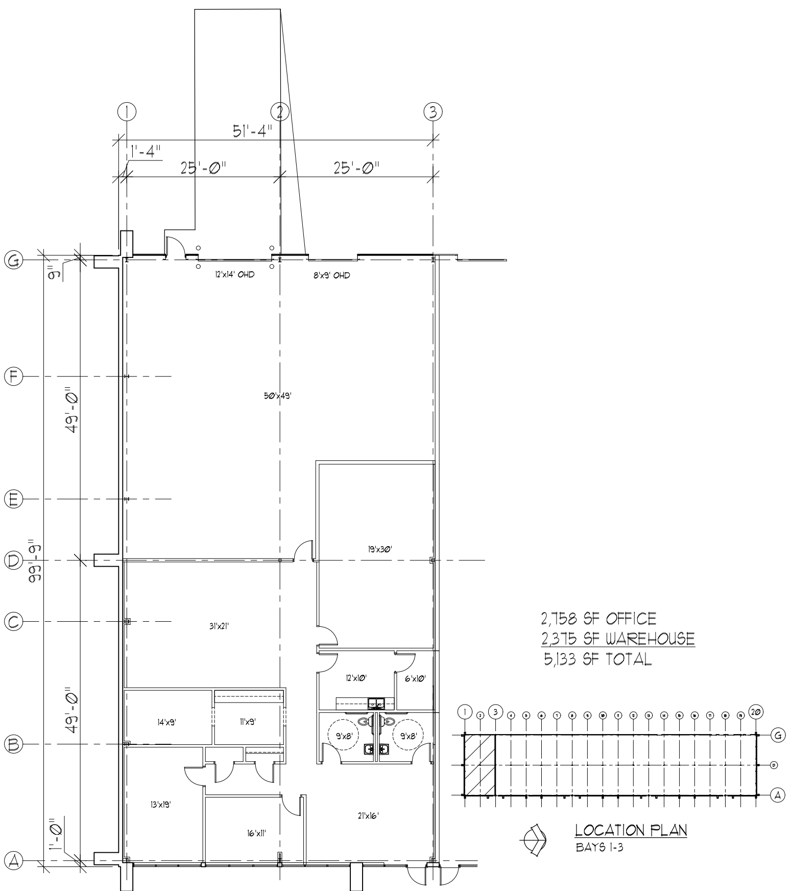
FLOOR PLAN BAYS 1-3
