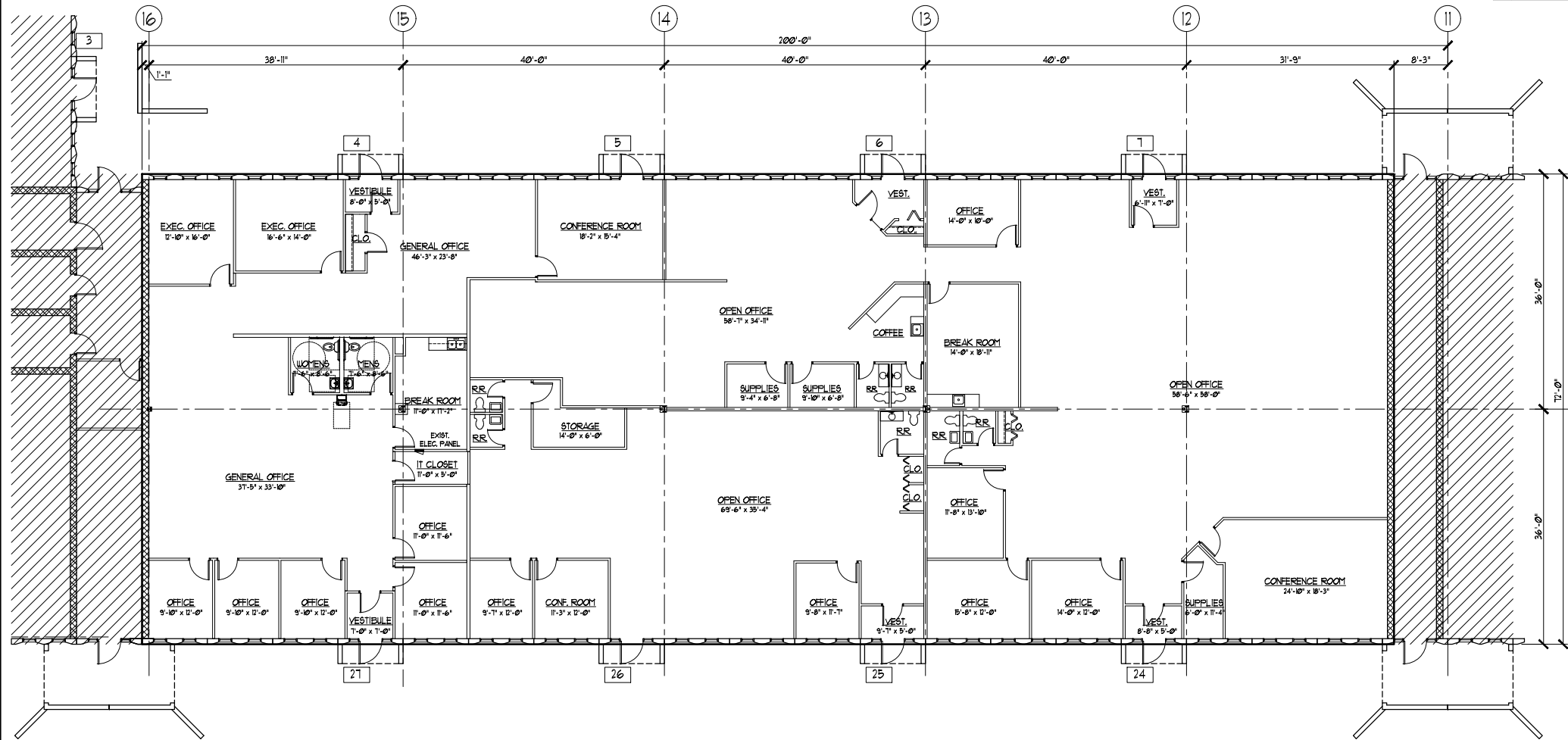
FLOOR PLAN 13,826 SF
