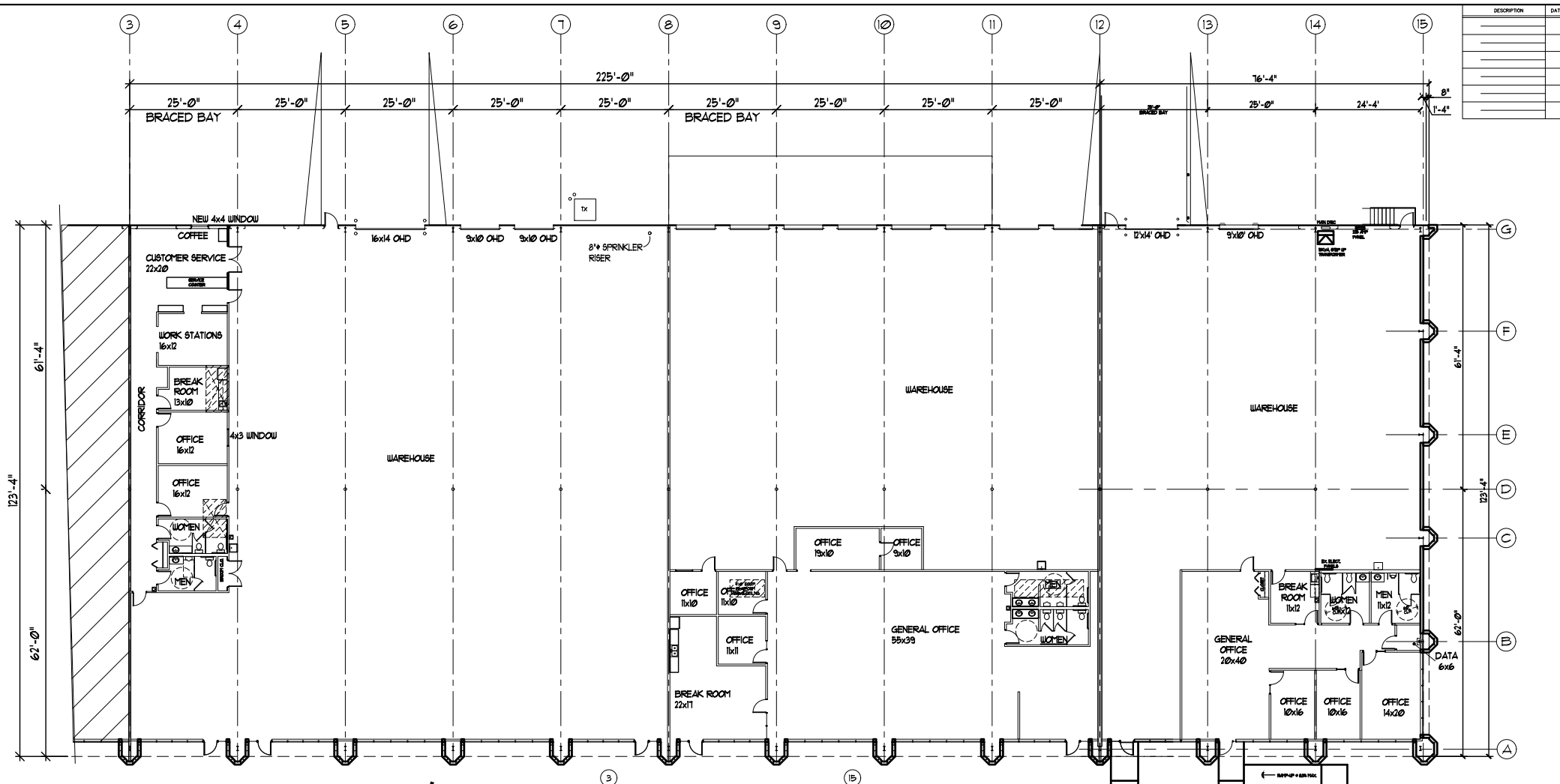
FLOOR PLAN
