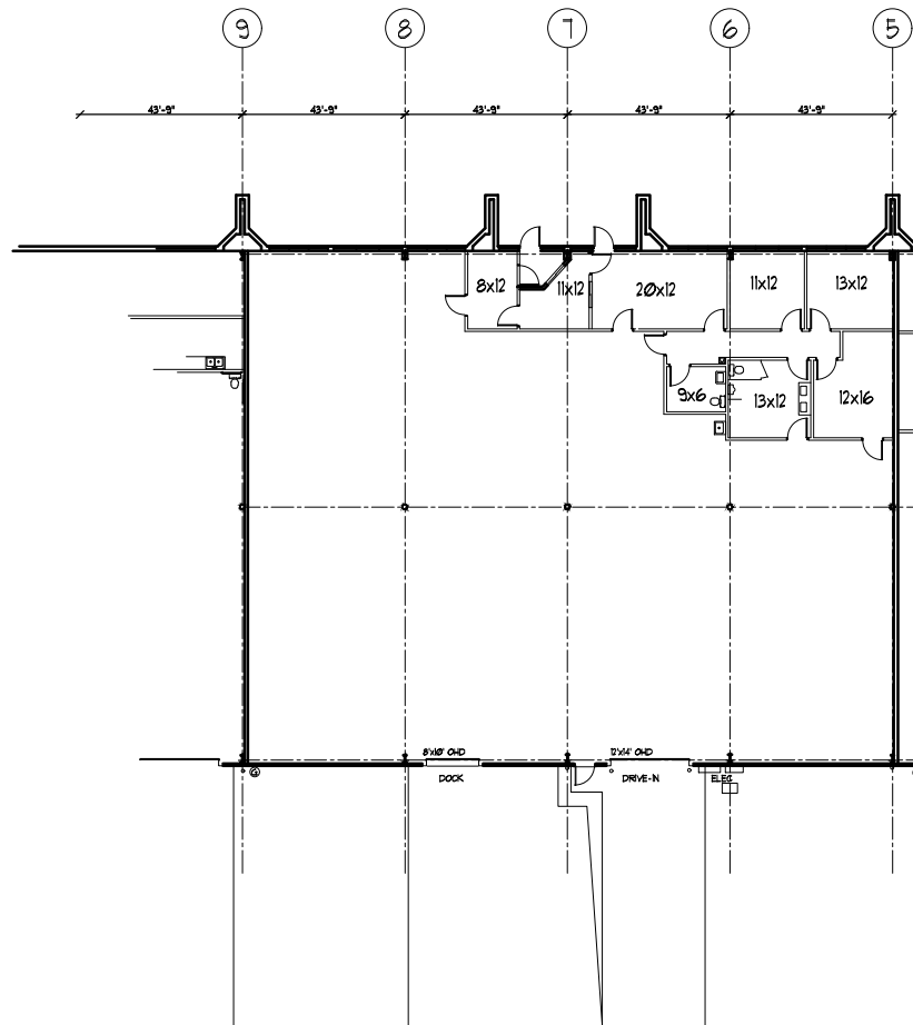
FLOOR PLAN
